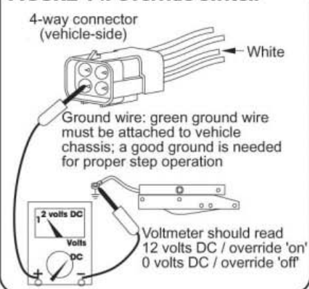
FIGURE 14: Override switch
