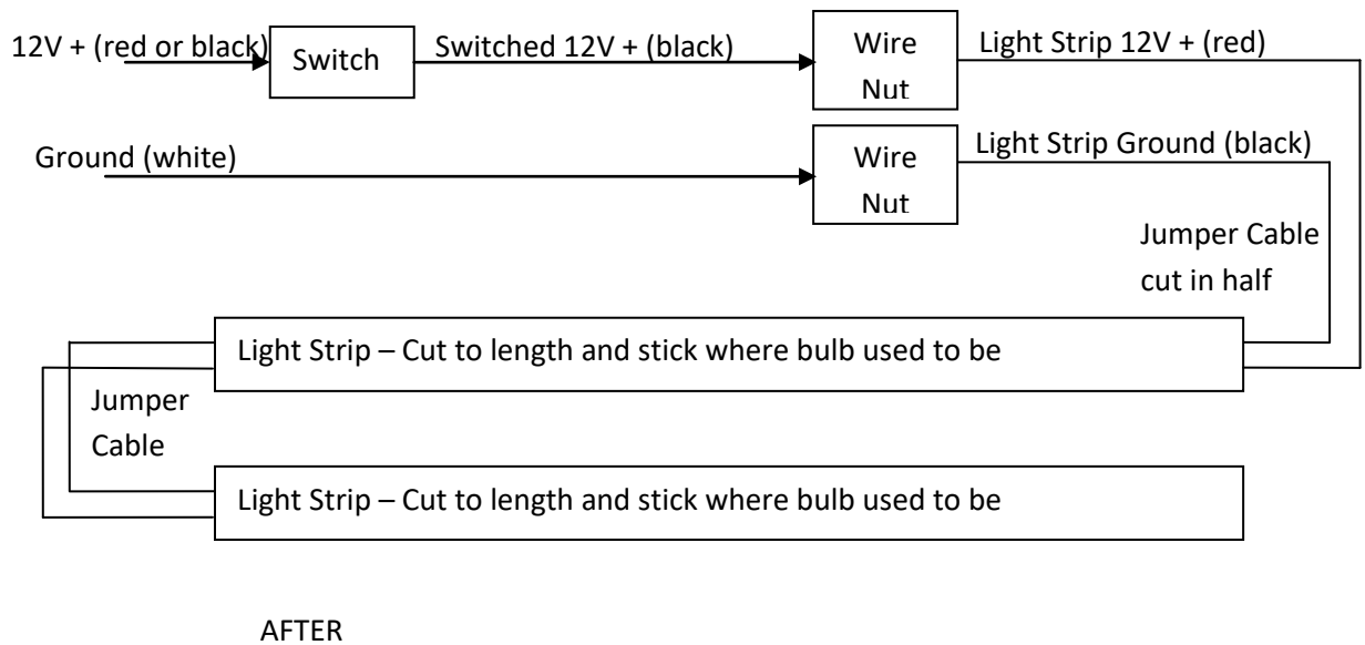
CHINOOK Fluorescent Replacement Wiring Diagram
