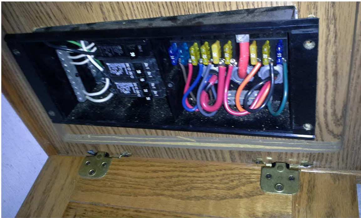
Todd Engineering LC30 Converter/charger and fuse panel are in two separate boxes
