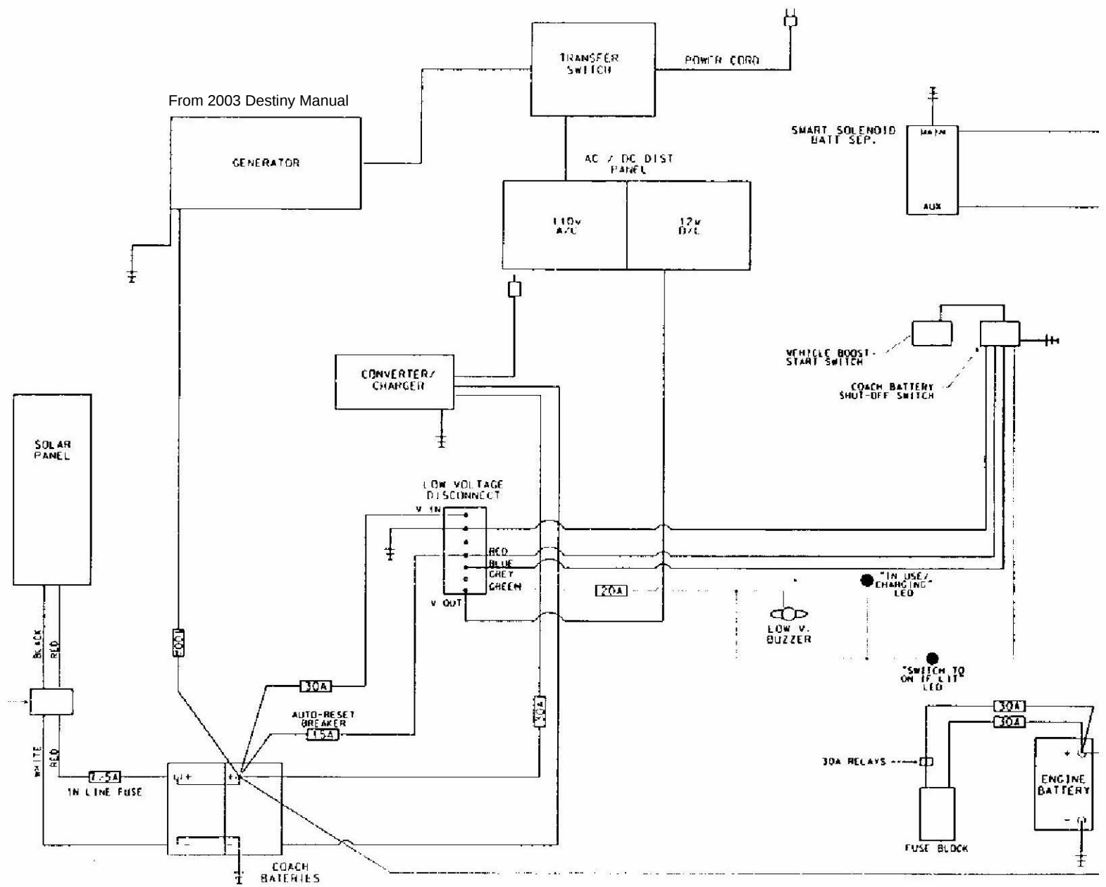
Todd Engineering LC30 Converter/charger and fuse panel are in two separate boxes
