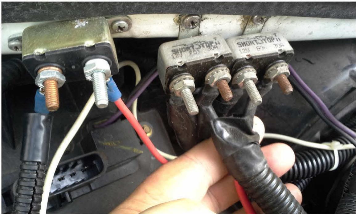
Positive terminal of battery, almost directly below my hand.
